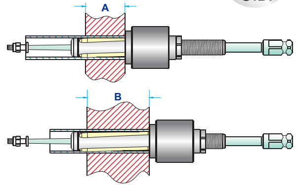
FOR TUBES INTERNAL DIAMETER FROM (8.4 mm) .334" TO (36.3 mm) 1.43"
